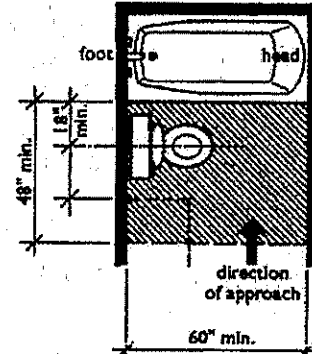
2 Specification "A" Bathrooms 48" X 60"
